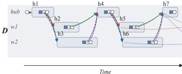
(a) the record: 7 activations of 3 agents, 8 deliveries
